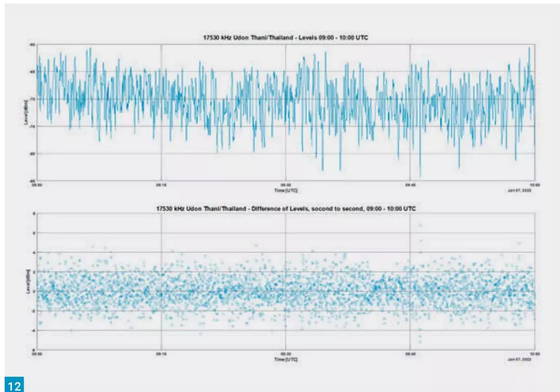
Fig. 12: Dynamic ionosphere leads to typical shortwave fading (top), which oscillates from second to second in the range of about \pm 4 dB [see text]. Fig. 13: The short-term dynamics and the information they contain are completely lost when the actual level curve is averaged at 110-second intervals – as it is done by logging WSPR signals.
