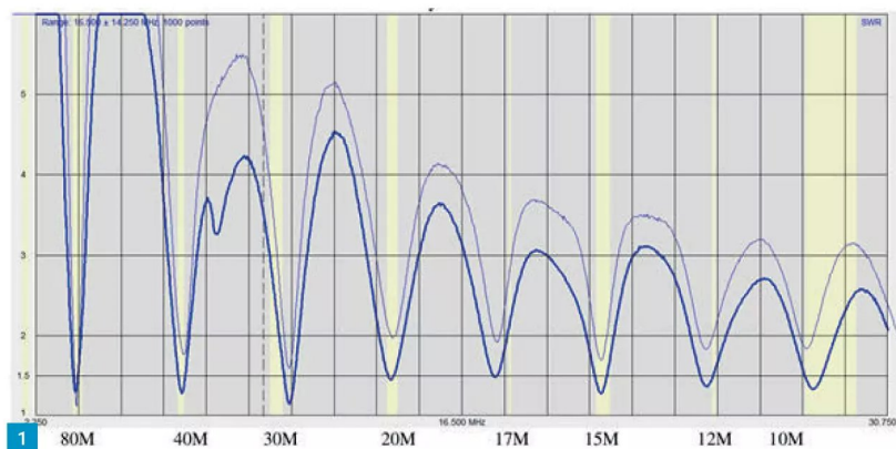
Fig. 1: RF Sweep of Horizontal HF Loop, 275 feet in length, 30 feet AGL, by Everett N4CY (Source: Everett Sharp N4CY, "Experimenting with different baluns on a 275' Horizontal Multi-Band Loop Antenna 80/40/30/20/17/15/12/10/6m," 7 June 2015 (personal communication)). Thin light blue line is 2:1 Balun with the thicker dark blue line is a 4:1 Balun. Measured at shack end of 50' RG-8X coax, not at the 'bare wire' feedpoint. Fig. 2: Author's house with #14 THHN wire loop run about 1in underneath the architectural shingles on top of plywood underpinning, feeding into the attic via soffit as noted. Note that the house roof has several peaks so the wire travels upward and downward following the path of the edge of the shingles. A TDR measurement found that the wire length is about 276 feet.
